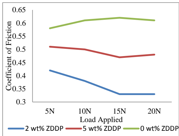
Figure 1 Coefficient of friction for corn oil with 0 wt%, 2 wt% and 5 wt% ZDDP.
