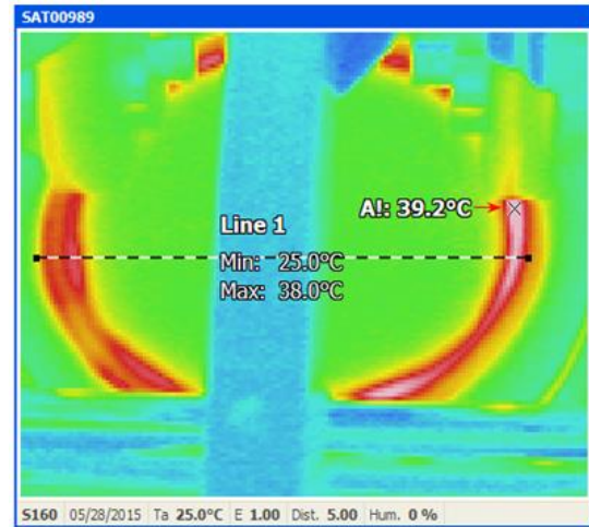
Figure 3 Thermal distribution at abrasion wheel.
