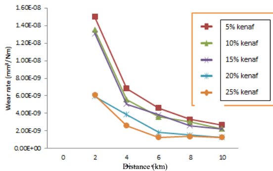
Figure 2 Specific wear rate of Kenaf composite over distance.
