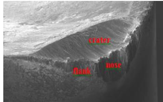
Figure 3 Wear on the uncoated carbide tool edge when turning Ti-6Al-4V ELI.
