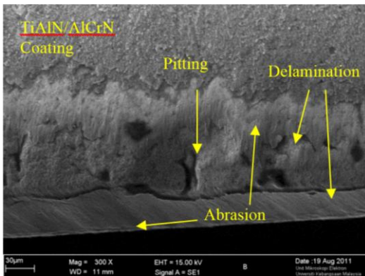
Figure 1 Several failure modes during machining of Inconel 718.
