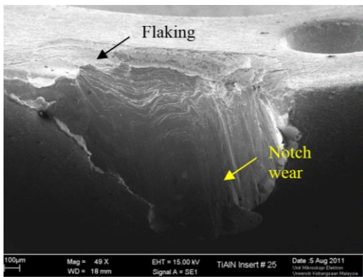
Figure 2 Failure mode observed during catastrophic failure.
