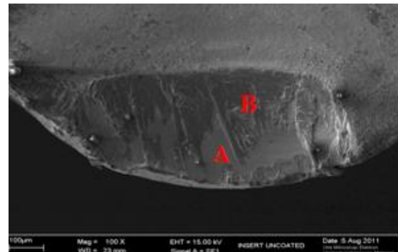
Figure 4 Crater wear on the top rake face of the tool; A) smooth wear area due to diffusion mechanism; B) melted titanium alloy.
