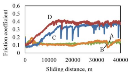
Figure 1 Friction coefficient with different moisture contents at 1MPa.
