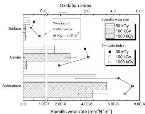
Figure 2 Specific wear rate of all testing surfaces.
