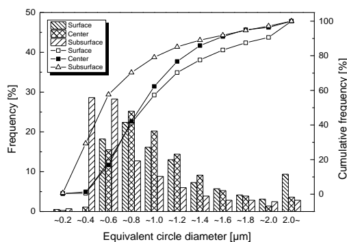
Figure 3 Size distribution of wear particles of 50 kGy cross-linked UHMWPE.
