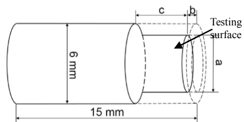
Figure 1 The geometry of pin sample.
