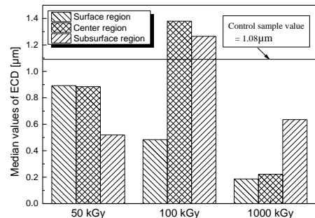
Figure 4 Median values of ECD of wear particles of all testing samples.
