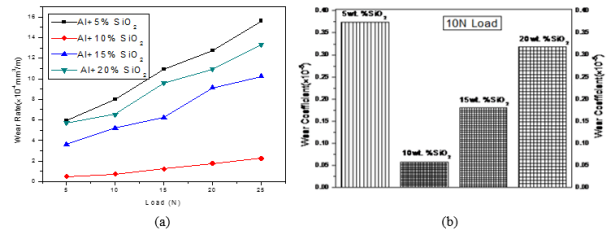
Figure 3 (a) Variation of wear rate with normal load (b) wear coefficient.
