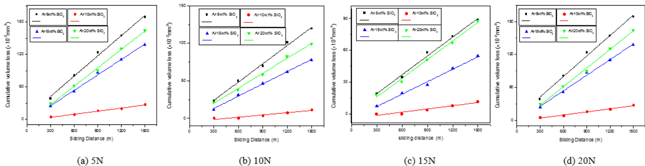
Figure 2 Variation of cumulative volume loss with sliding distance.
